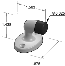
DS-1 – Floor mount door stop. – Includes mounting hardware for wood & masonry floors.
