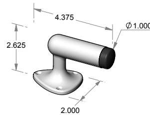
DS-2EXT – Floor mount door stop. – Includes mounting hardware for wood & masonry floors.
