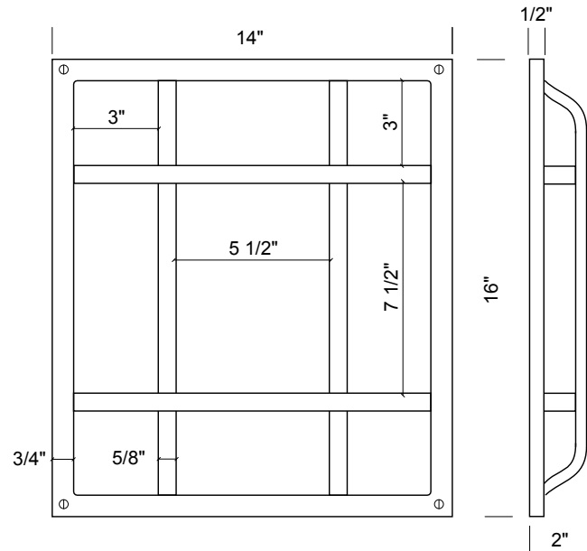
SEG-1416 – Speak easy grill. – Available 5/8" wide flat grill only.
