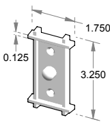
DRB-751 – Trellis door bell plate. – Matching solid bronze button.
