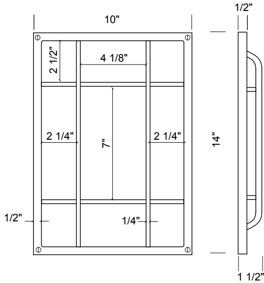
SEG-1014 – Speak easy grill. – Available 1/4" round grill only.
