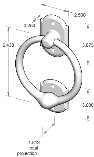
DKA-6 – Door knocker w/strike plate.
