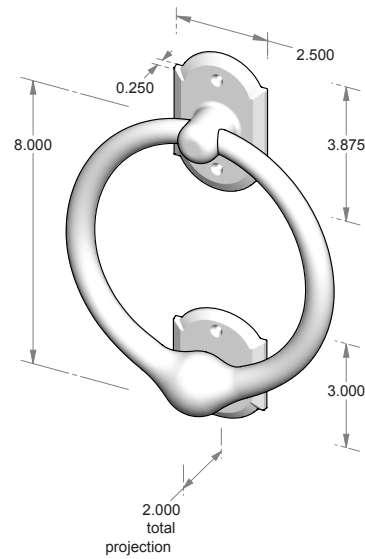
DKA-8 – Door knocker w/strike plate.
