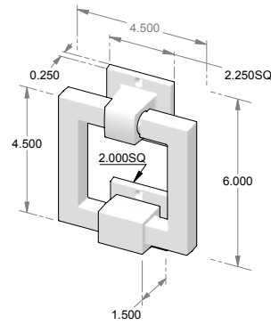
DK-94 – Square door knocker w/strike plate.
