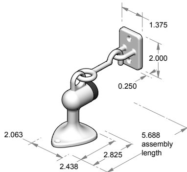
DS-2HE – Floor mount door stop w/hook & eye. – Includes mounting hardware for wood & masonry floors.
