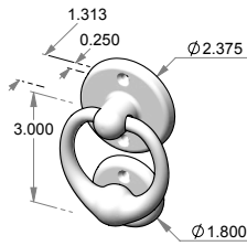
DK-3 – Door knocker w/strike plate.
