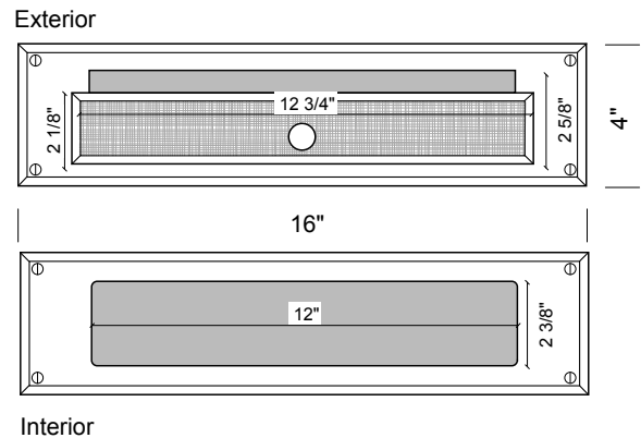
CS-MLST-2216 – Mail slot with Burlap door. – Includes interior trim.
