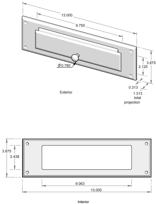
CS-MLST-13 – Mail slot with door. – Includes interior trim.
