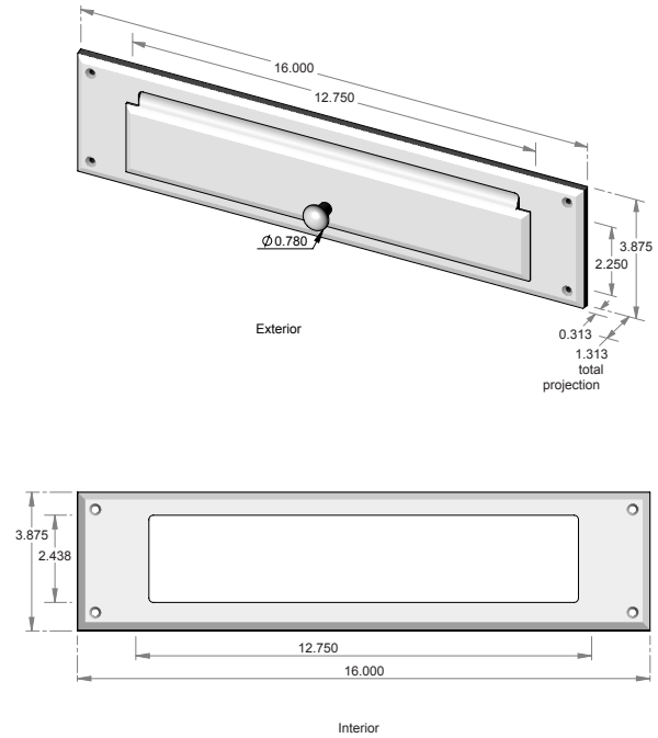
CS-MLST-16 – Mail slot with door. – Includes interior trim.
