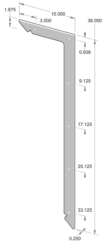
SH-C-36 – Decorative corner bracket. – Right hand shown.
